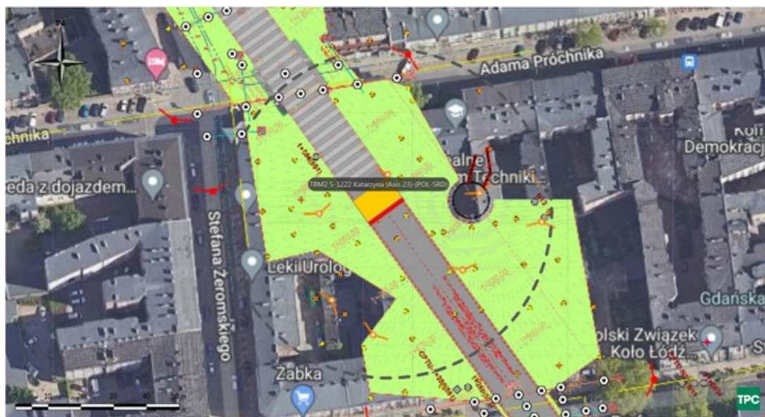
Figure 1-2 Plan view of TBM Position on 02/09/2024
