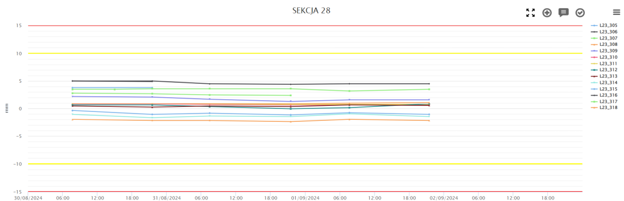
Figure 6-2 Settlement of Section on Prochnika street
