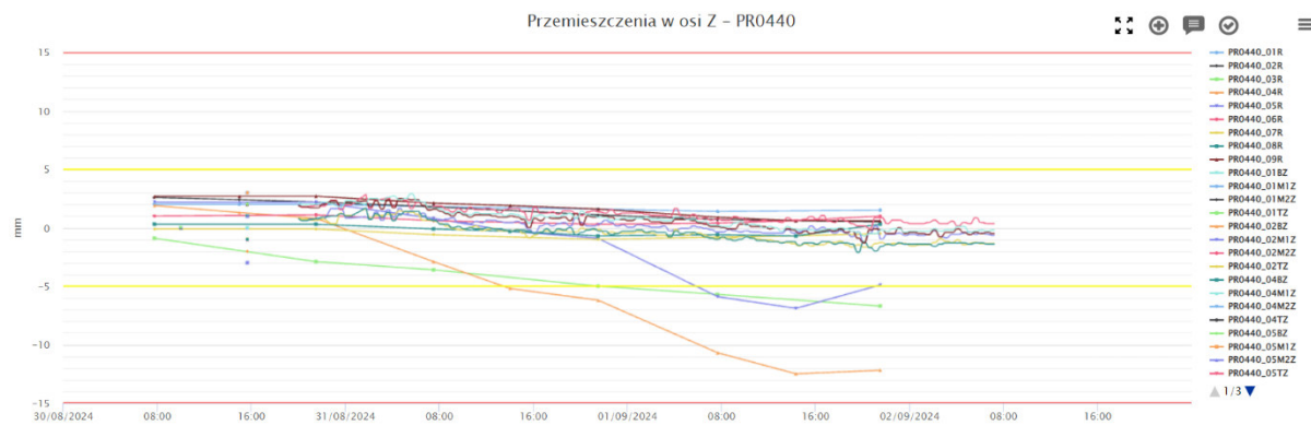
Figure 6-4 Settlement of building PR0440
