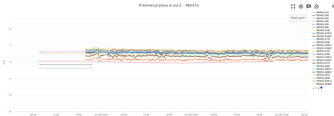
Figure 6-5 Settlement of building PR0450
